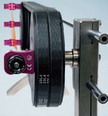
攜帶型皮帶輪雷射對心儀 G-PLUS Pulley Laser Alignment Pack
