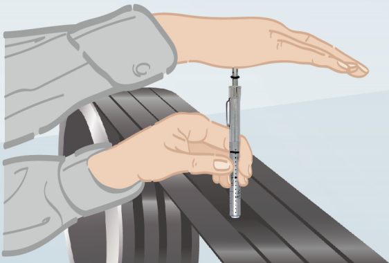
筆型皮帶張力計 Belt Tension Meter
