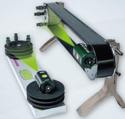
綠G光皮帶輪雷射對心儀 GL-2000 Belt Pulley Alignment Tool
